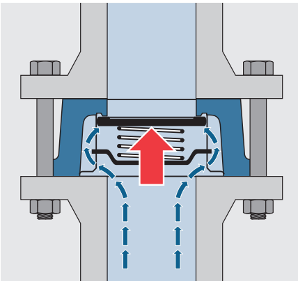
GESTRA DISCO® non-return valve in the closed state
