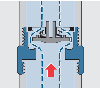
Pump running, normal operation
