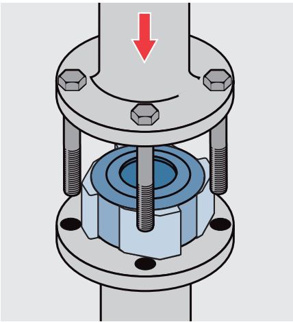
GESTRA DISCO® non-return valve with self-centering body, DN 15–100 ( 1/2–4")
