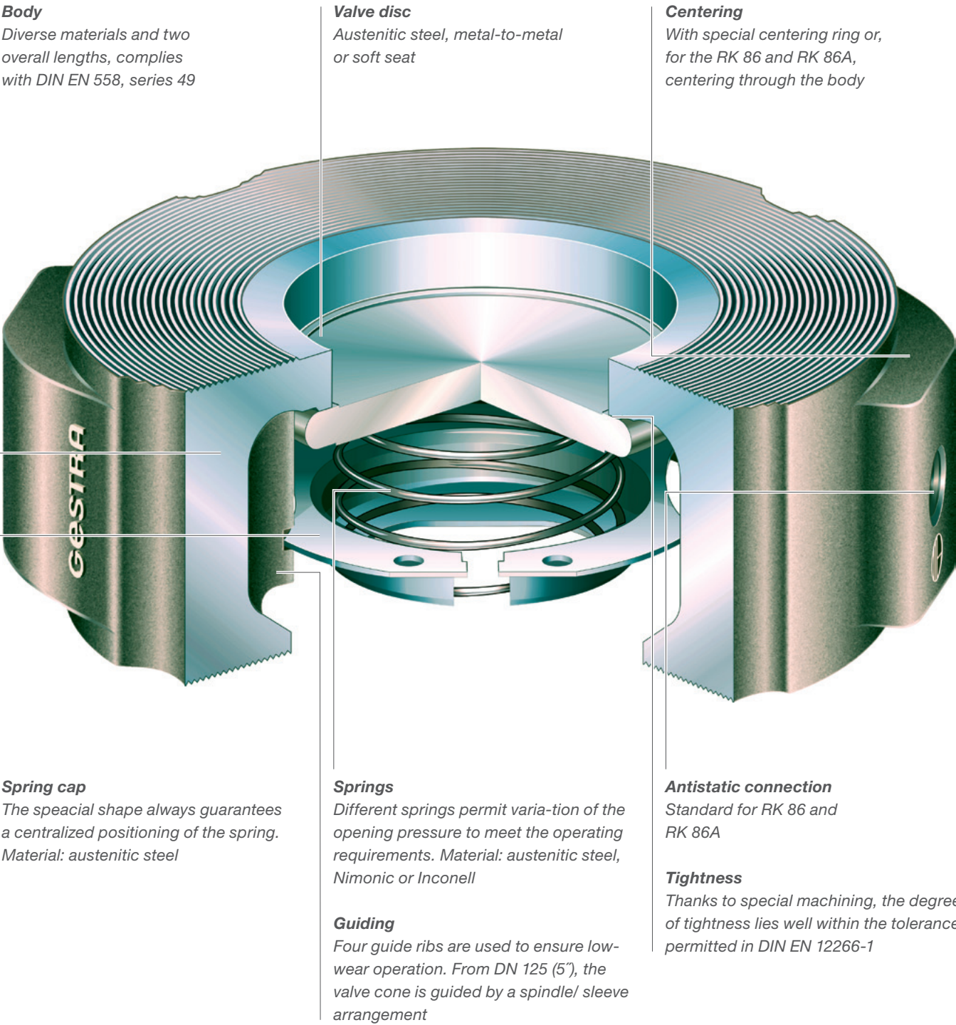
RK 86/RK 86A DN 15 up to 100
